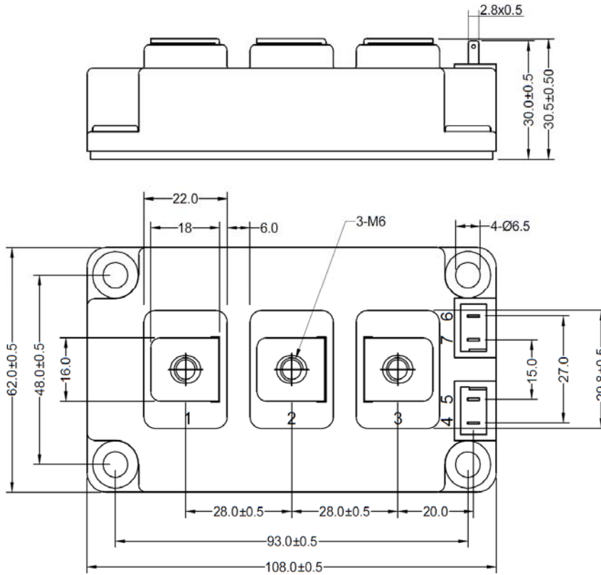
Dimensions in (mm) Figure 14. Package Outline
