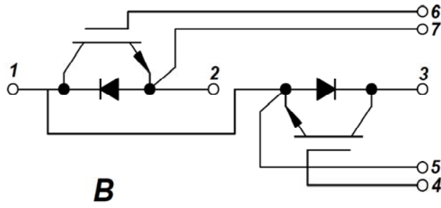
Figure 13. Circuit Diagram
