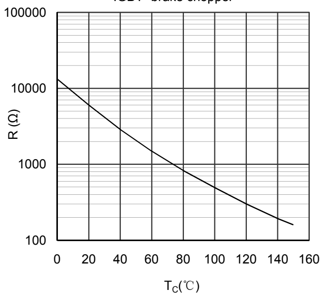
Figure 14. NTC Characteristics
