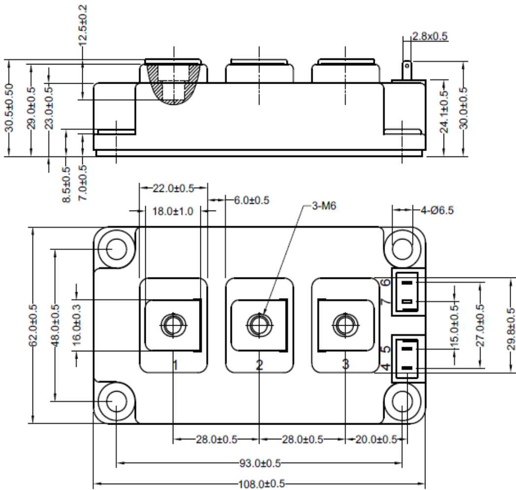
Dimensions in (mm) Figure 14. Package Outline
