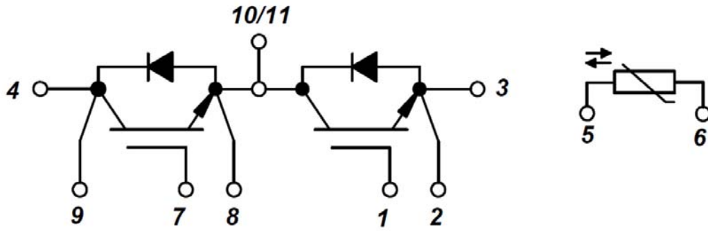
Figure 14. Circuit Diagram
